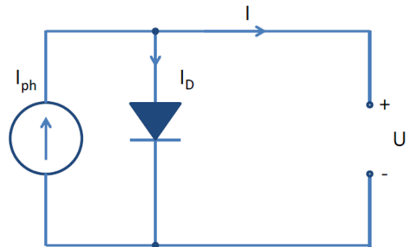
Figure 2 Real PV cell
